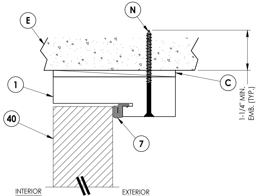
5 7 VERTICAL CROSS SECTION Shown Direct to Masonry
