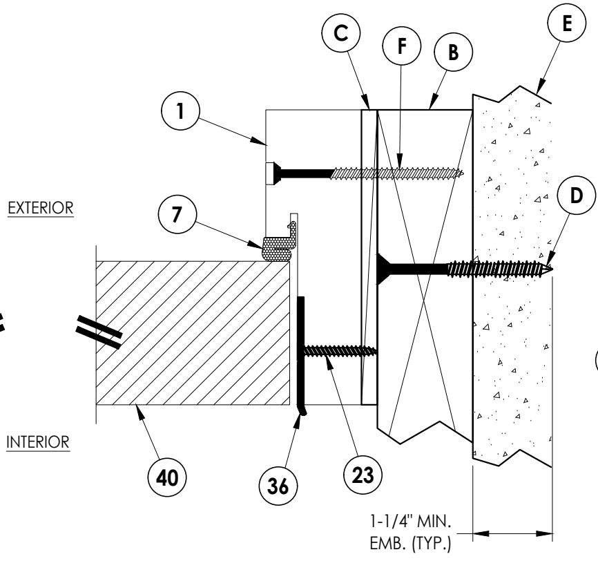
2 5 HORIZONTAL CROSS SECTION 2X Buck Construction
