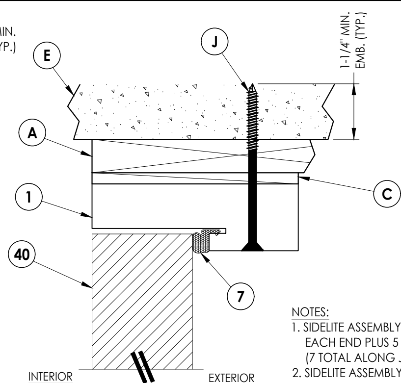
5 6 VERTICAL CROSS SECTION 1X Buck Construction
