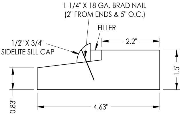
4 WOOD SIDELITE SILL
