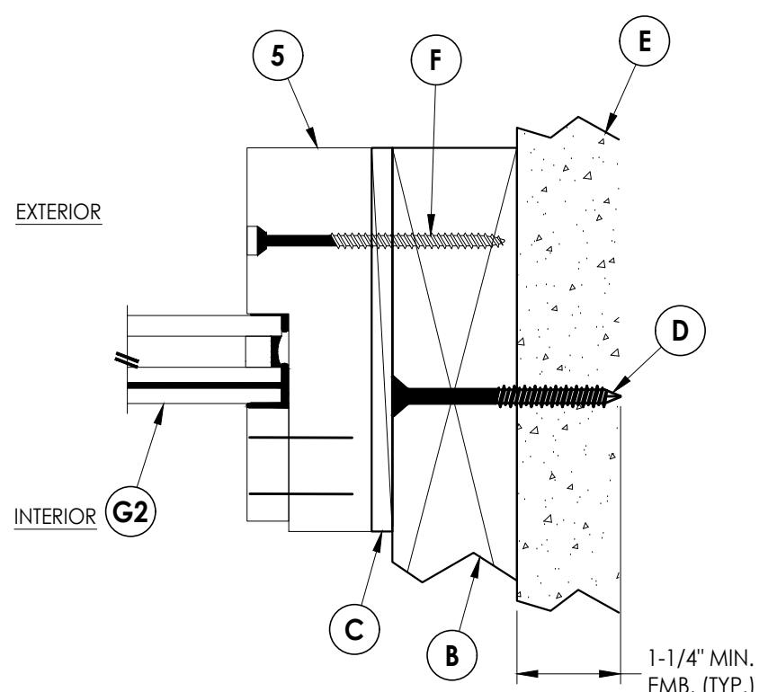
4 5 HORIZONTAL CROSS SECTION 2X Buck Construction
