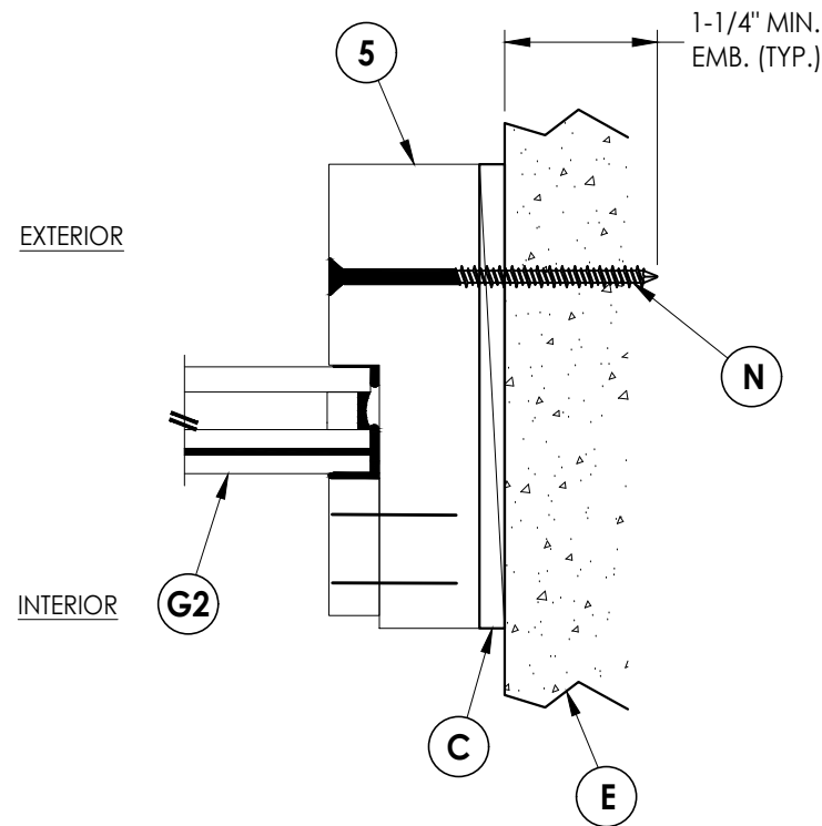
4 7 HORIZONTAL CROSS SECTION Shown Direct to Masonry
