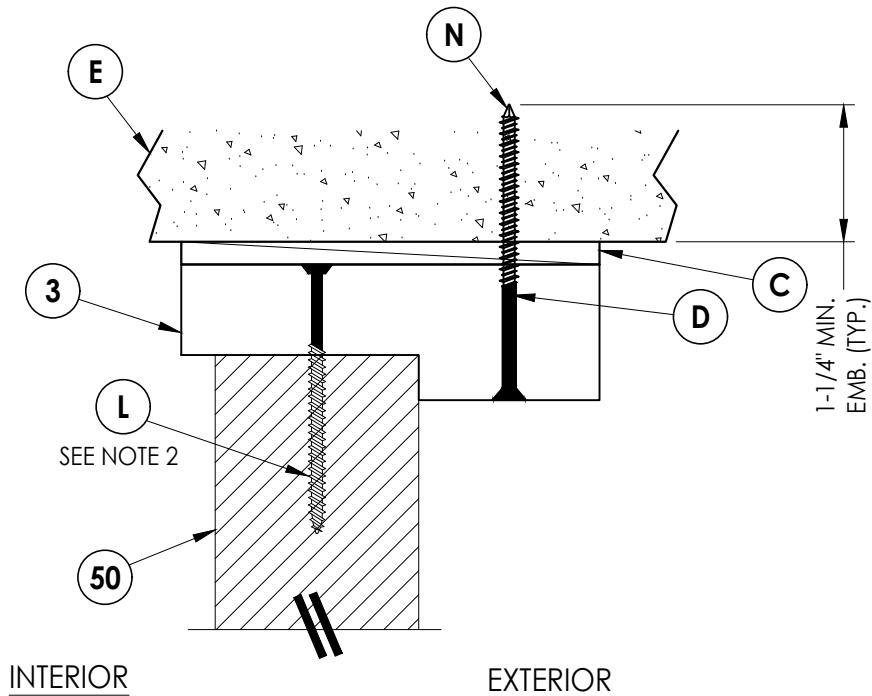
6 7 VERTICAL CROSS SECTION Shown Direct to Masonry
