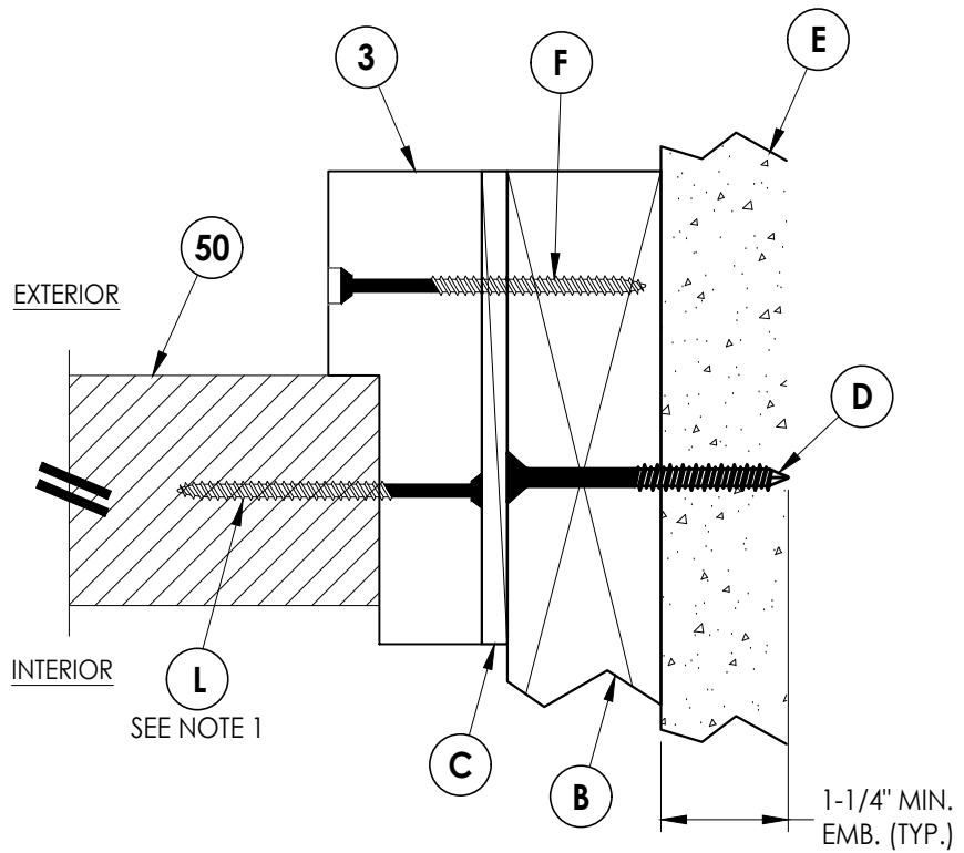
3 5 HORIZONTAL CROSS SECTION 2X Buck Construction
