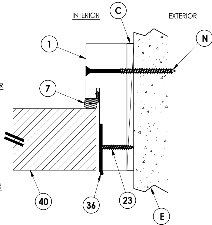
2 7 HORIZONTAL CROSS SECTION Shown Direct to Masonry
