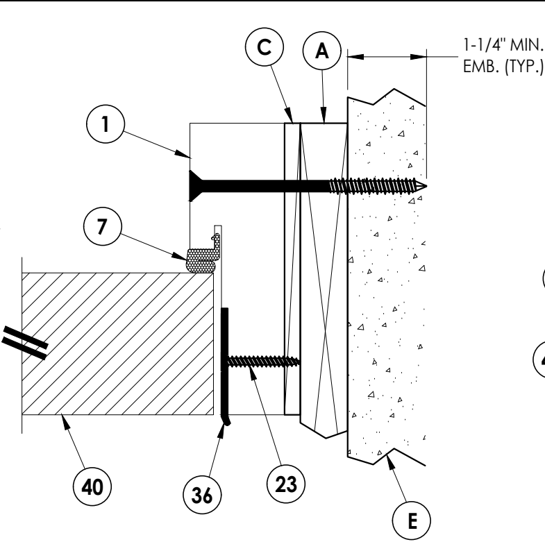
2 6 HORIZONTAL CROSS SECTION 1X Buck Construction
