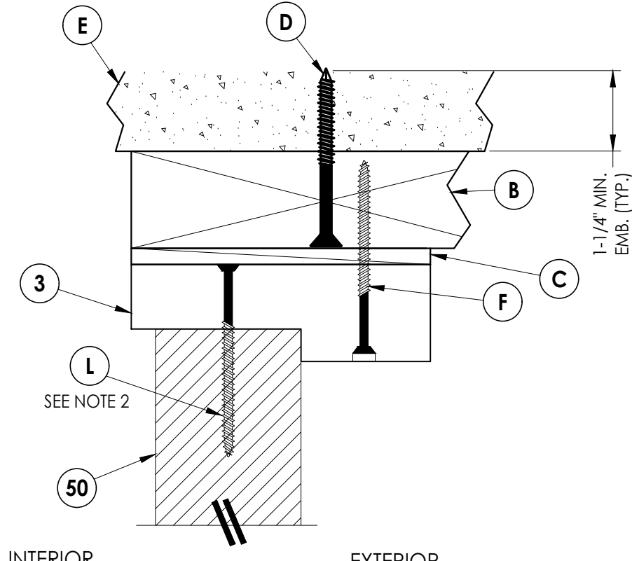
6 5 VERTICAL CROSS SECTION 2X Buck Construction
