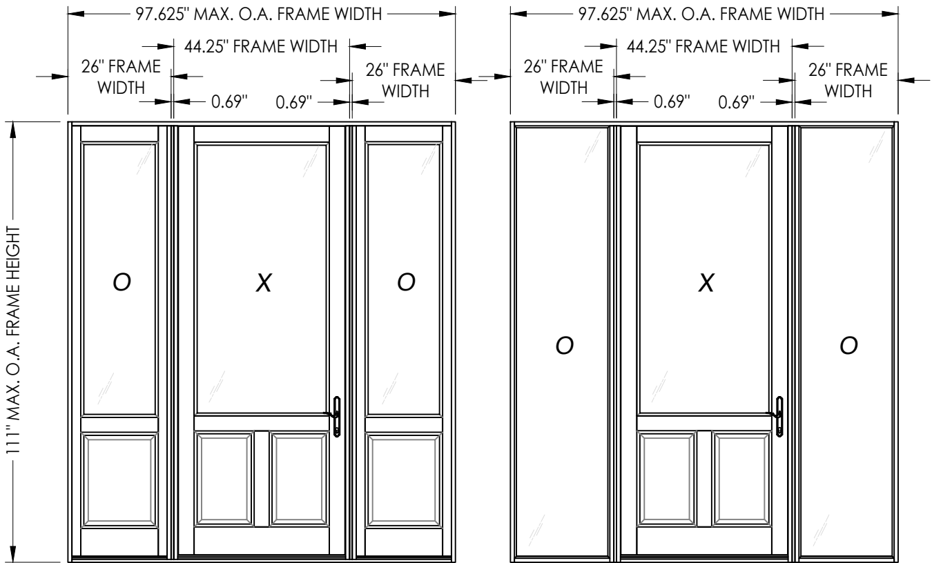
SHOWN w/ 3/4 LITE SIDELITES
