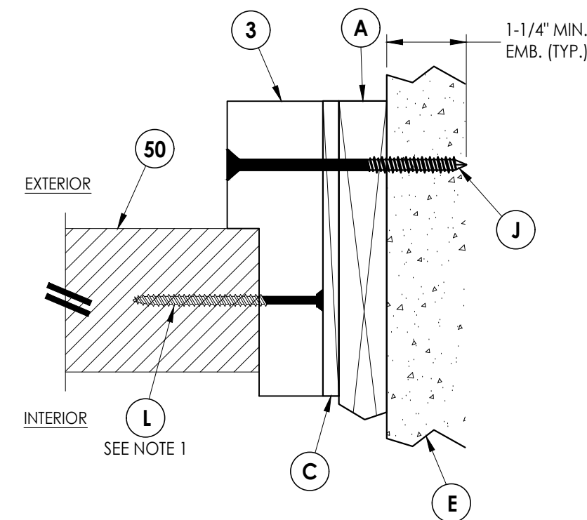
3 6 HORIZONTAL CROSS SECTION 1X Buck Construction
