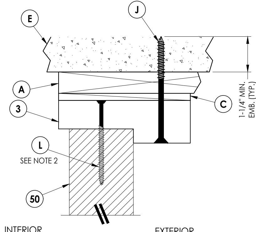
6 6 VERTICAL CROSS SECTION 1X Buck Construction
